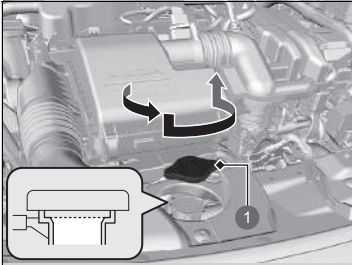
1 Radiateurdop
