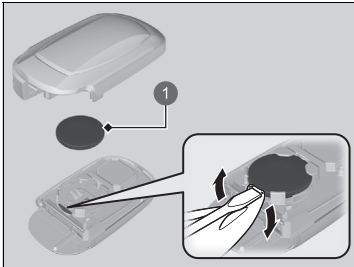
1 Accu
